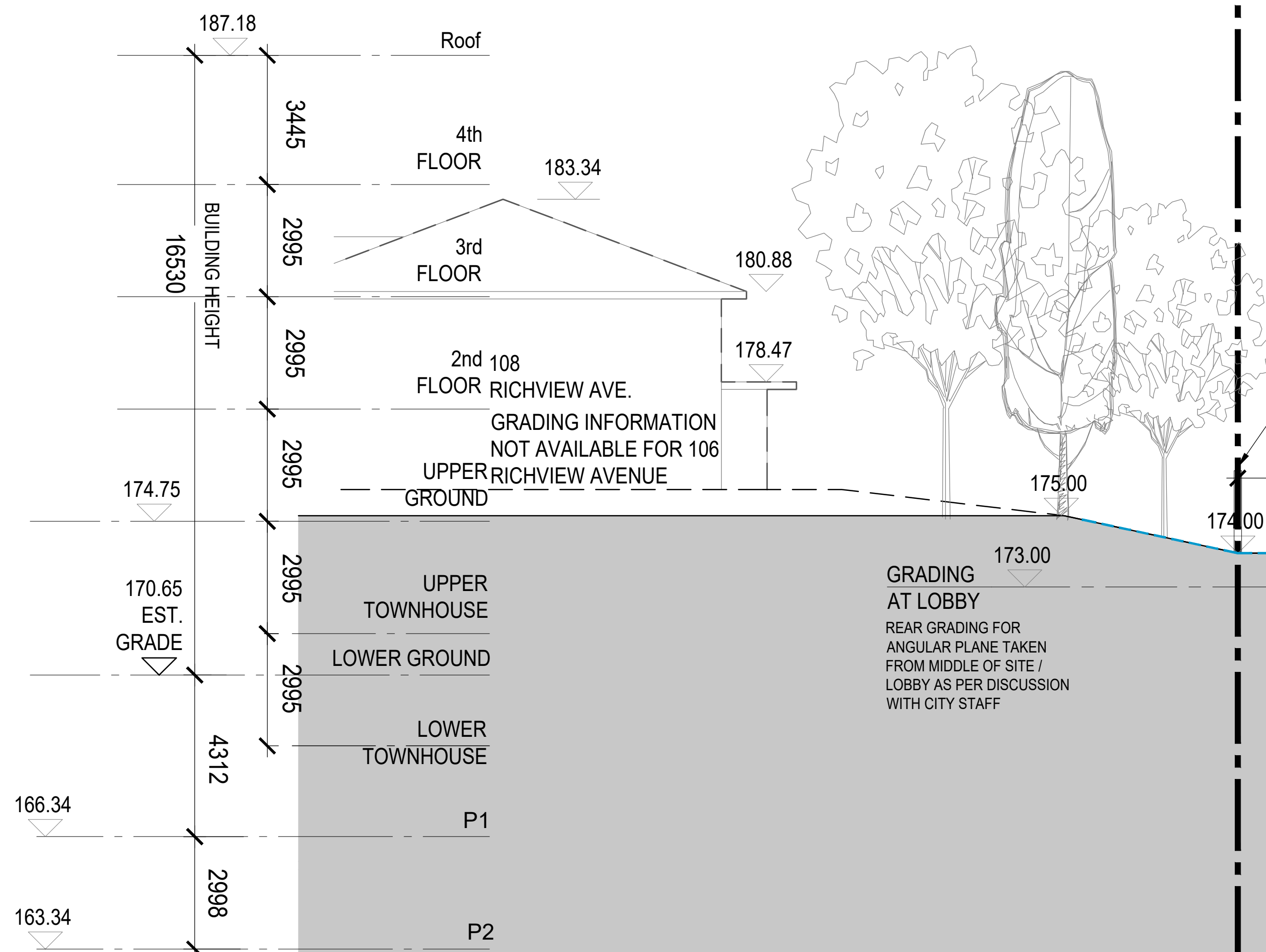
SECTION G-G'
