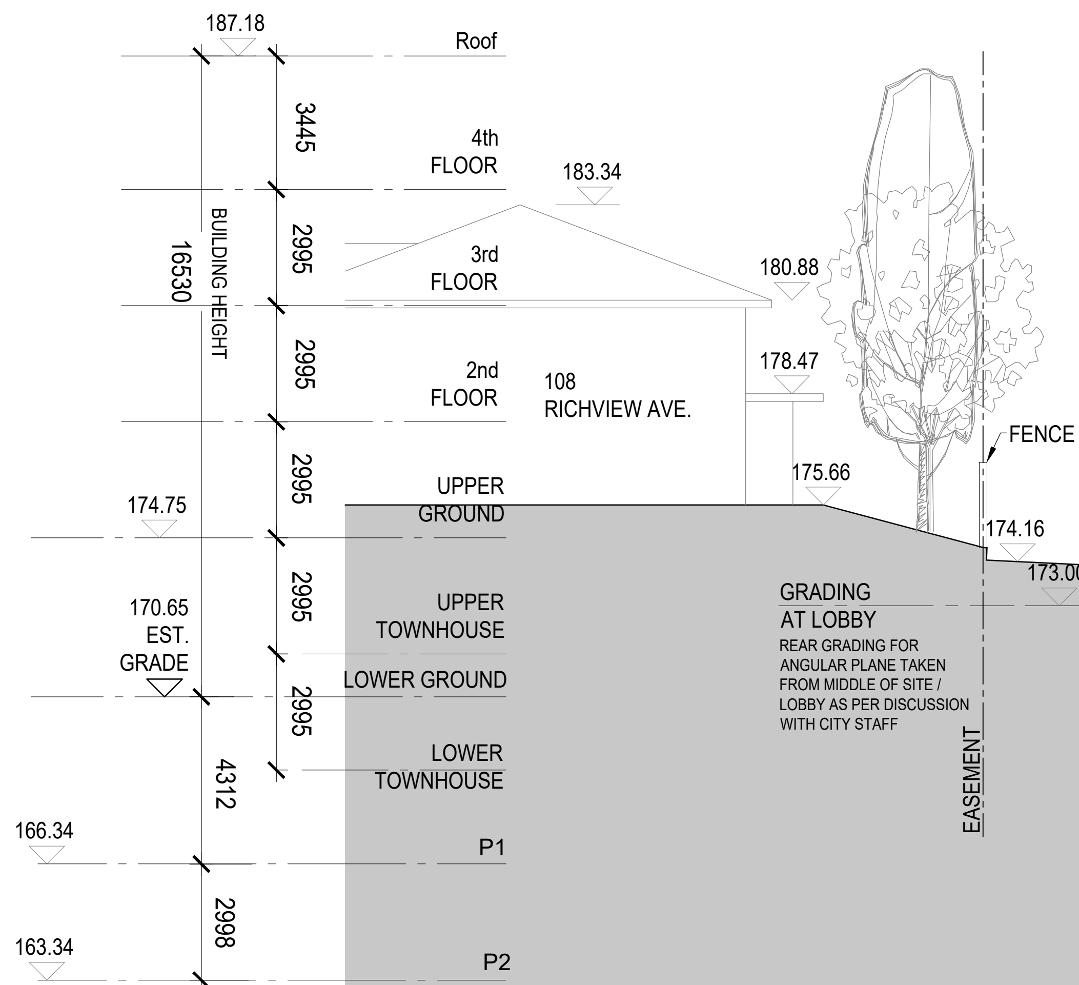
SECTION F-F
